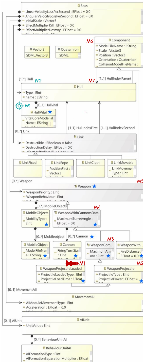
Fig. 4 Fragment of the metamodel which describes the rules for creating bosses in Kromaia. The elements marked with stars indicate the parts of such excerpt which are involved in the Equipment Configuration step. The series of marks M1-M7 and W1-W2 are examples which show the elements involved in terms of support for missiles (a type of weapon) and weak points, respectively, beyond Equipment Configuration.
