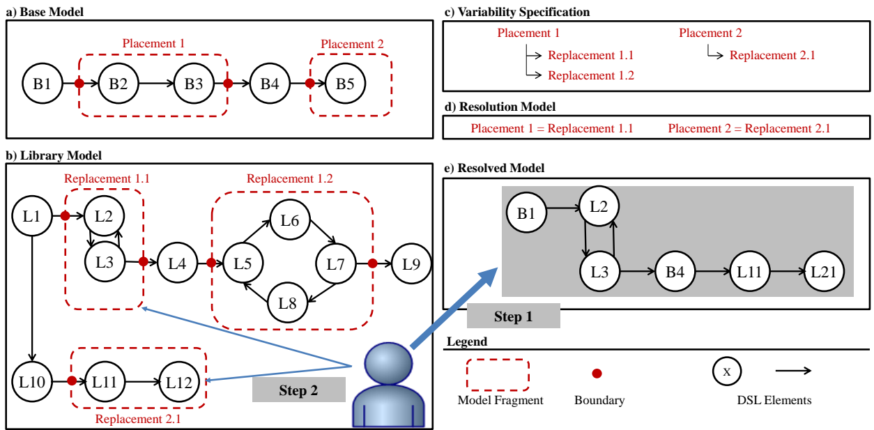
Figure 4. Visualization task
