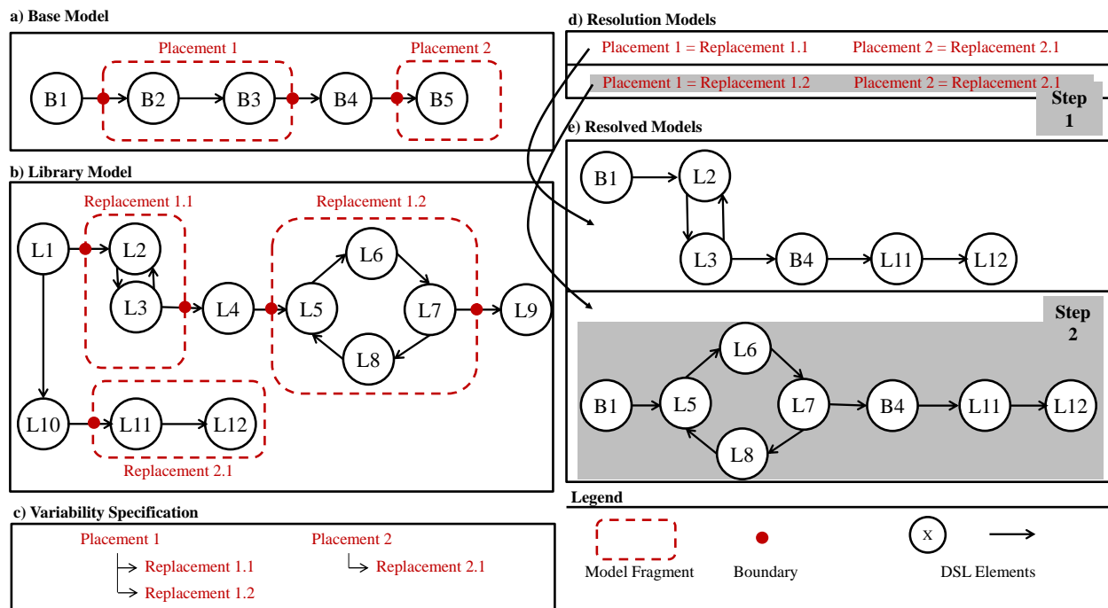
Figure 2. Configuration task
