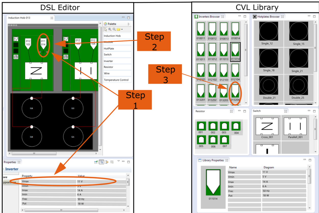
Figure 9. Scope task
