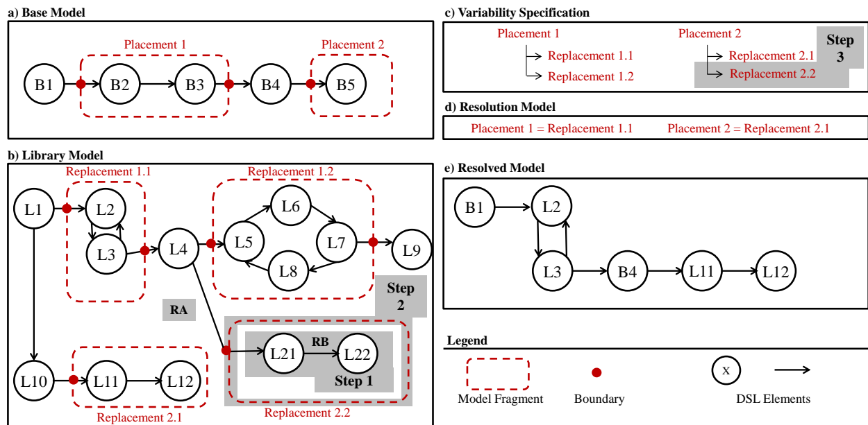
Figure 3. Scope task
