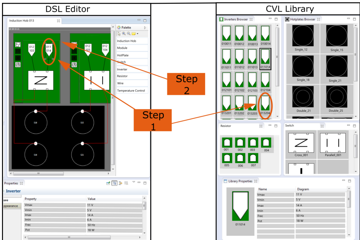
Figure 8. Configuration task
