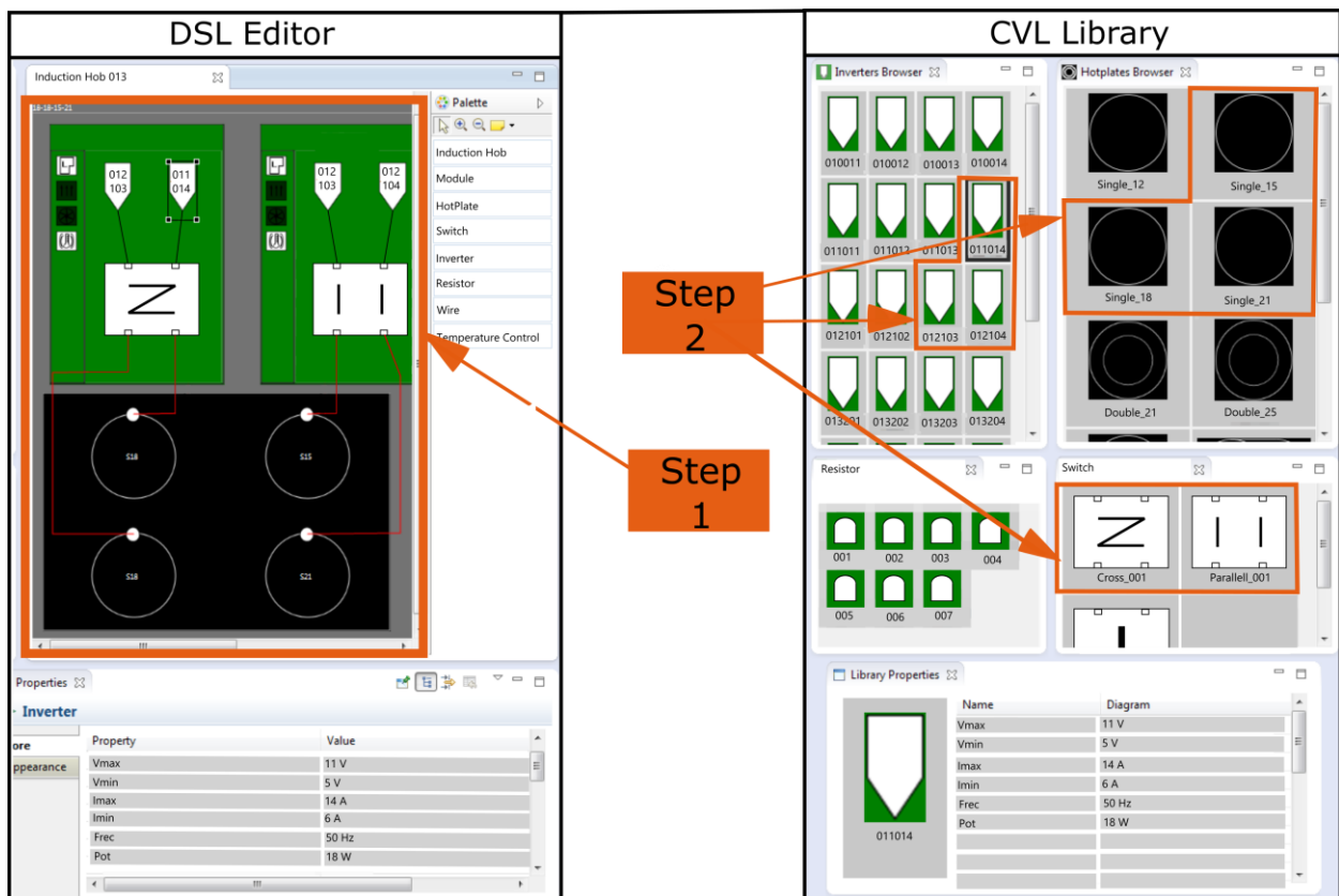
Figure 10. Visualization task
