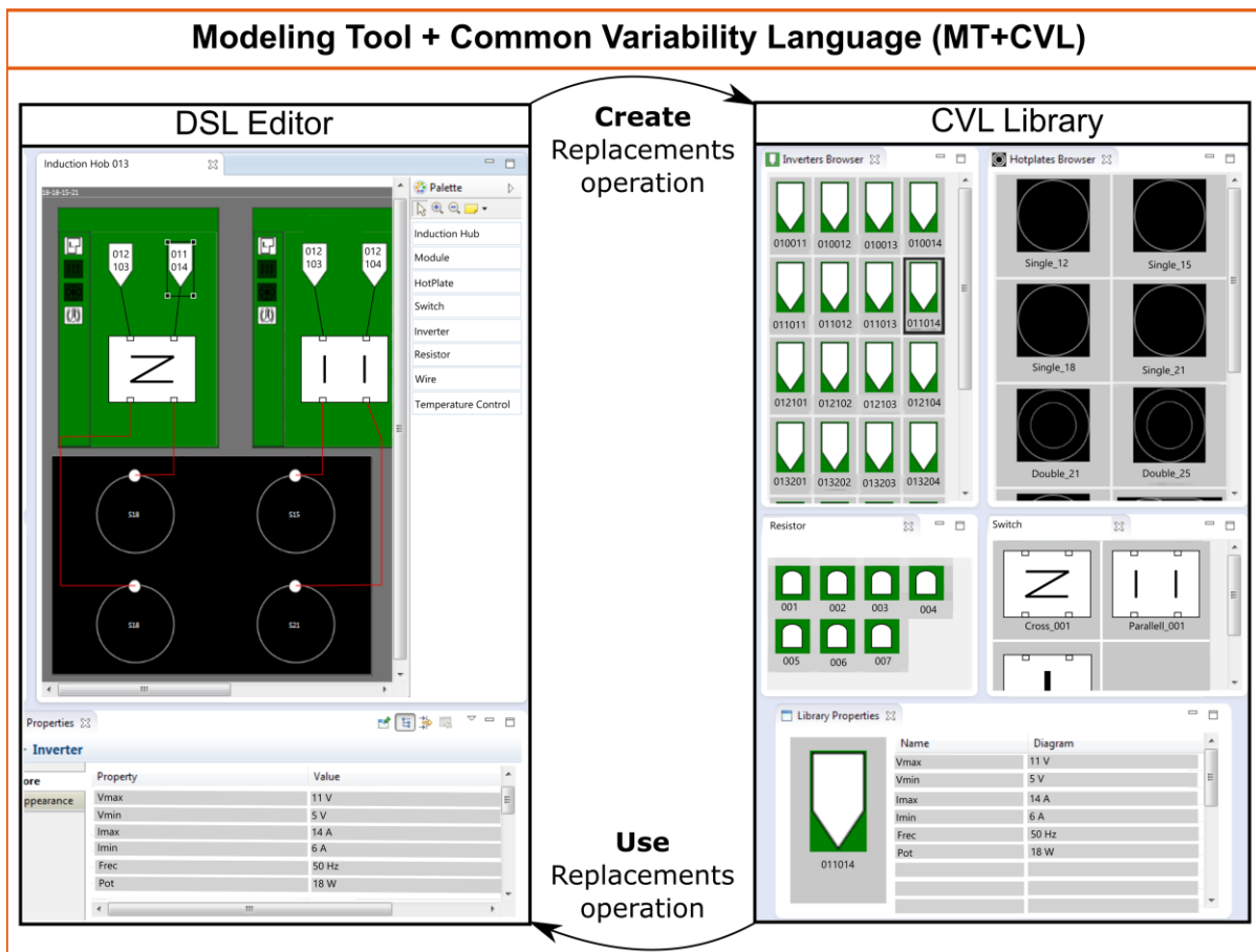
Figure 7. Induction Hob MT+CVL
